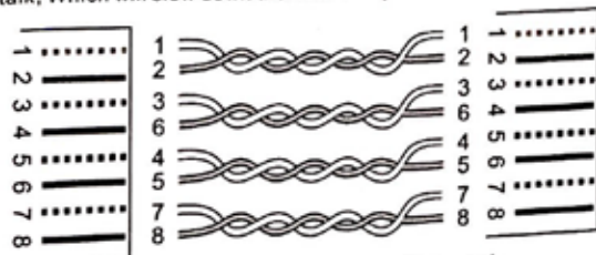
Connection diagram of crosstalk line pair
