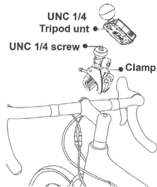
Fig. 8 Bike application
