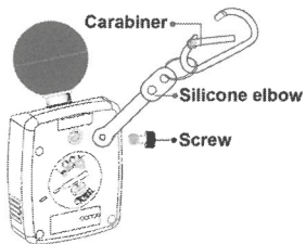
Fig. 3 Hanging kit
